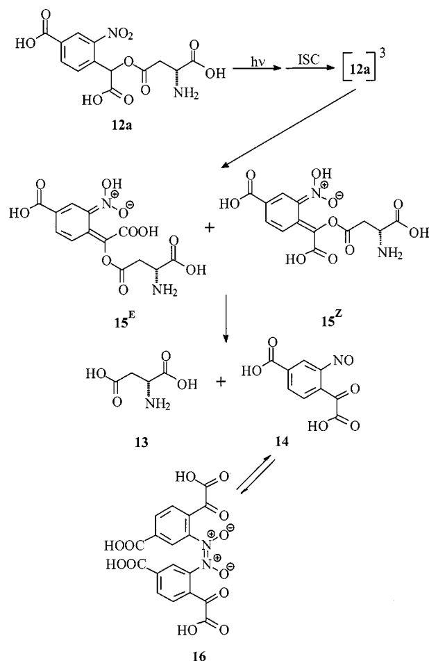
Scheme 4. Proposed mechanism of photolysis of \beta -DCNB-D-aspartate
