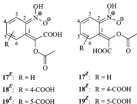
Scheme 5. Model compounds used in our ab initio studies
