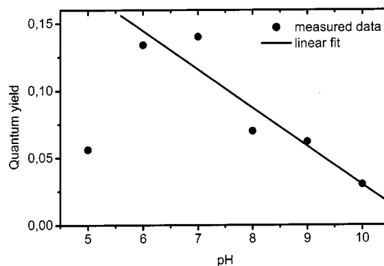
Figure 6. The quantum yield for the photorelease of aspartate from \alpha ,4-DCNB-aspartate 12a (500 \mu M) is shown (filled circles); a linear fit (straight line) for pH \geq 6 is shown; below pH = 6 the quantum yield becomes smaller again
