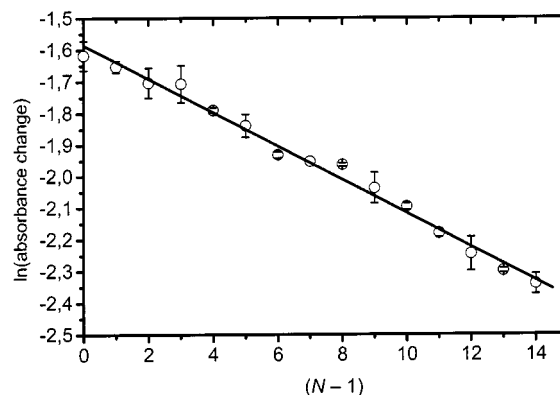
Figure 5. A sample of \alpha ,4-DCNB-aspartate 12a (500 \mu M, 100 mM phosphate buffer, pH = 7.0, 50 \mu L) was irradiated with consecutive laser pulses (10 ns, 308 nm, 10 mJ); the logarithm of the transient absorption immediately after the laser pulse (0.5 \mu s) was plotted versus the number of the laser pulses - 1; from the slope of this linear fit we obtained the quantum yield and from the intercept we were able to estimate the extinction coefficient of the aci -nitro intermediate; each data point represents the mean of three experiments
