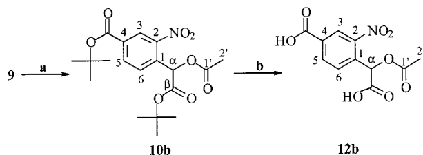
Scheme 3. Synthesis of the model compound DCNB-acetate 12b . a: DBU, THF, HOAc 63 %, b: TFA, toluene, 59 %
