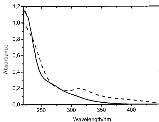
Figure 3. UV/Visible spectrum of 12a (50 \mu M, 100 mM phosphate buffer, pH 7.1) before photolysis (straight line) and of the reaction products (dashed line) after complete photolysis (100 laser pulses of 15 mJ, 330 \mu L solution)
