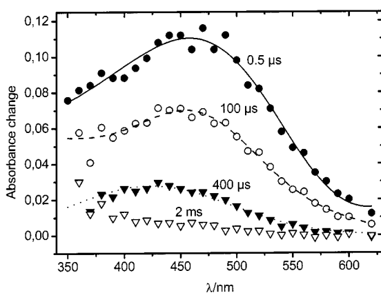
Figure 2. UV/Visible spectra of the transient absorption recorded 0.5 \mu s, 100 \mu s, 400 \mu s, and 2 ms after the laser flash; the spectra were constructed from several transient spectra, recorded at wavelengths of 350 to 630 nm (stepwidth 10 nm)
