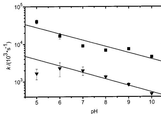
Figure 4. pH-Dependence of the rate constants of the fast ( k_1 ) and the slow ( k_2 ) exponential components of the decay of the aci -nitro intermediates 15
