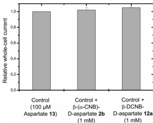
Figure 7. Whole-cell current recording for EAAC1 expressed in HEK293 cells with 100 \mu\text{M} free aspartate 13 (column 1), 100 \mu\text{M} free D-aspartate 13 in the presence of 1 mM \beta -( \alpha -CNB)-D-aspartate 2b (column 2), and 100 \mu\text{M} free D-aspartate 13 in the presence of 1 mM \beta -( \alpha ,4-DCNB)-D-aspartate 12a (column 3)
