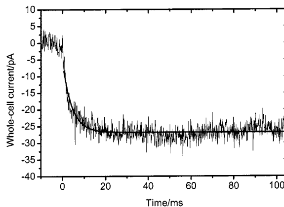
Figure 8. Laser-pulse photolysis experiment with 150 \mu\text{M} \beta -( \alpha ,4-DCNB)-D-aspartate 12a ; aspartate was released upon application of a 345 nm, 10 ns laser pulse (400 mJ/cm 2 ); the current was recorded at U = 0 \text{ mV} ; the liberated D-aspartate concentration was estimated as 15 \mu\text{M}
