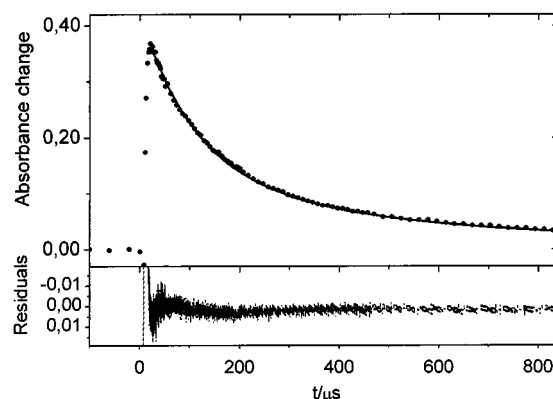
Figure 1. The transient absorption upon irradiation at t = 0 \text{ s} of 1 mM \beta -caged \alpha ,4-DCNB aspartate at pH = 7 (100 mM phosphate buffer); the sample was irradiated with a 10-ns laser flash at 308 nm and the absorption was measured at 430 nm; the solid line presents the best fit of the data ( A_0 = 0.013 , A_1 = 0.27 , t_1 = 105 \text{ } \mu\text{s} , A_2 = 0.13 , t_2 = 42 \text{ } \mu\text{s} ), the filled circles represent the measured data (1 out of 50 data points is shown), the lower panel shows the residuals of the fit
